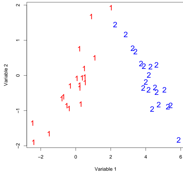
Figure 4: Scatter plot of the bivariate toy data; two clusters are generated, the first cluster from a standard bivariate Gaussian distribution with correlation 0.9 the second with mean (4, 0)^T , \rho = -0.9 , and unit marginal variances.
