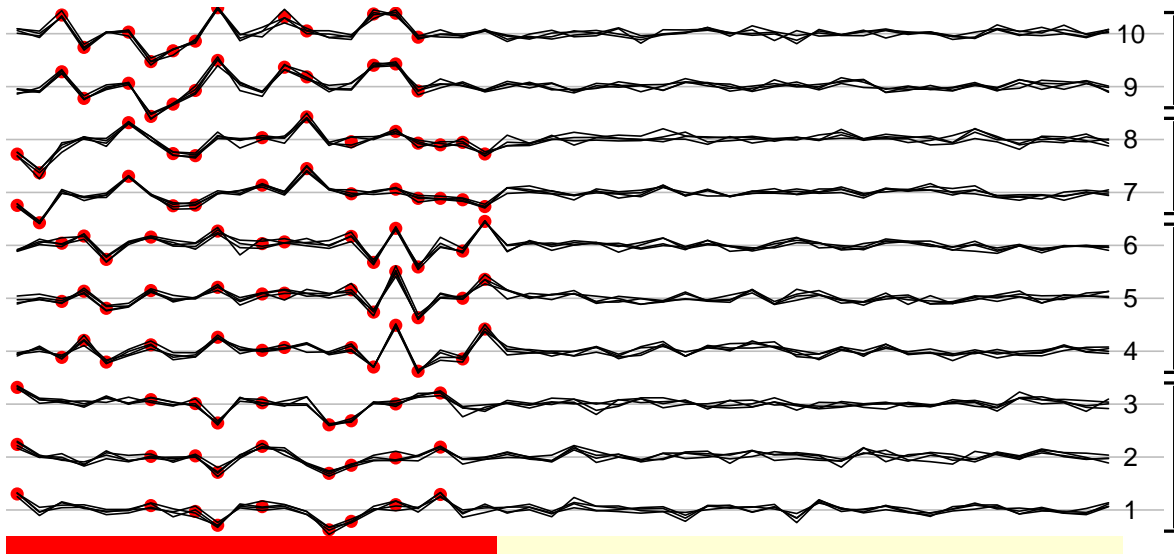
Figure 5: Profile plot of data simulated using the Gaussian model with 10 clustering individuals, each having four replicates over 50 variables. The hyper-parameter values are \sigma_\varepsilon^2 = 1, \sigma_\eta^2 = 1, \sigma_\theta^2 = 25, \mu = 0, p = 0.5, q = 0.5 . Four clusters are generated. The 22 activated variables are shown using the red horizontal bar. Activated variable-cluster combinations are shown using the red blobs on the profiles for each group.
