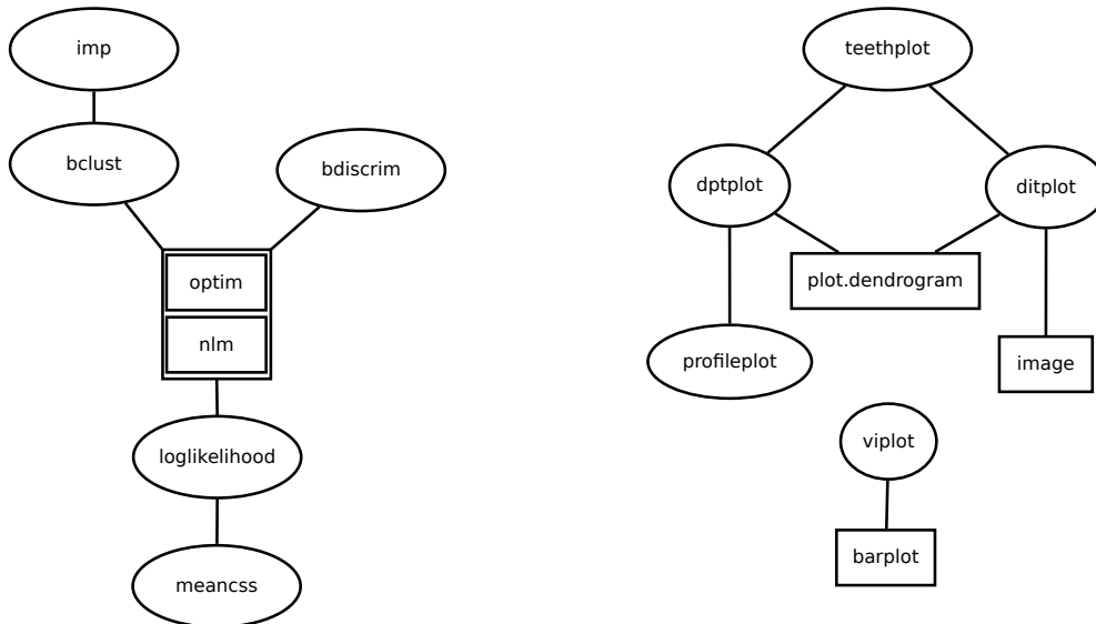
Figure 3: Diagram of function dependencies. Left panel: functions used for computations. Right panel: functions used for visualization. Ellipses denote functions developed in the bclust package and rectangles denote pre-existing R functions.
